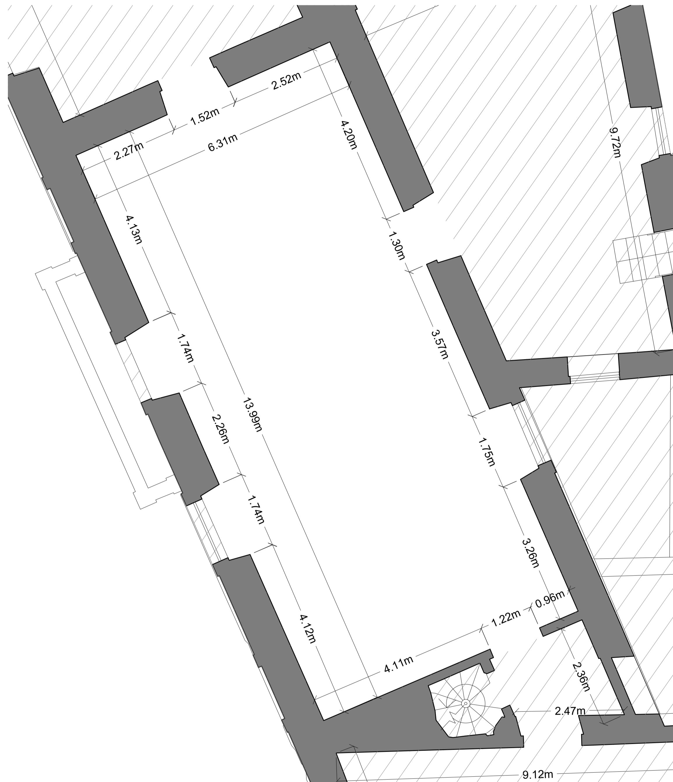
INQUISITOR'S PALACE - BELVEDERE ROOM SCALE 1:50
