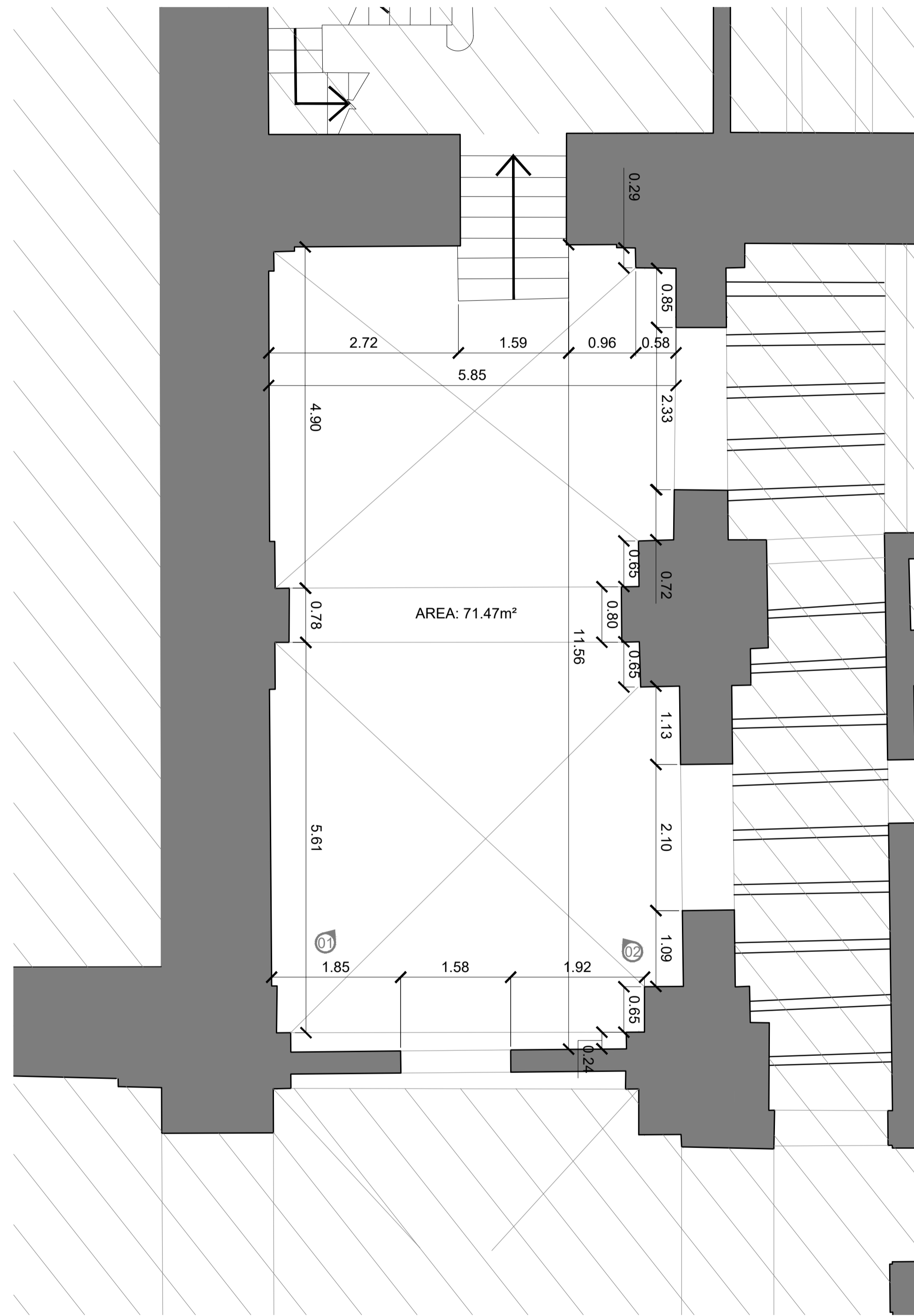
NATIONAL MUSEUM OF ARCHAEOLOGY GROUND FLOOR PLAN SCALE 1:50
